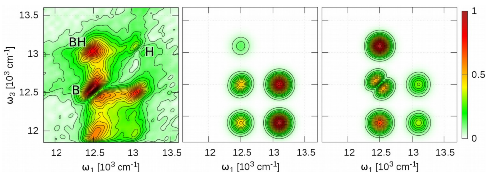
Fig. 1. All-parallel oscillation map at 560 cm -1 . Left: experimental oscillation map of rephasing real 2D signal, center: modeled pattern expected from normal stimulated emission and ground state bleach contributions, right: modeled interference between ground state bleach and ETICS signals reproducing cancellation on the diagonal.
